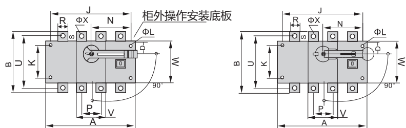
RDH5-125A~630A/JK柜外操作
